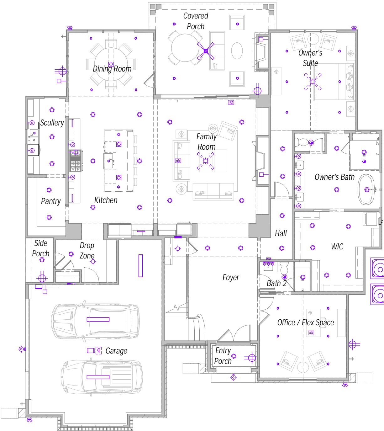
Main Level Electrical
